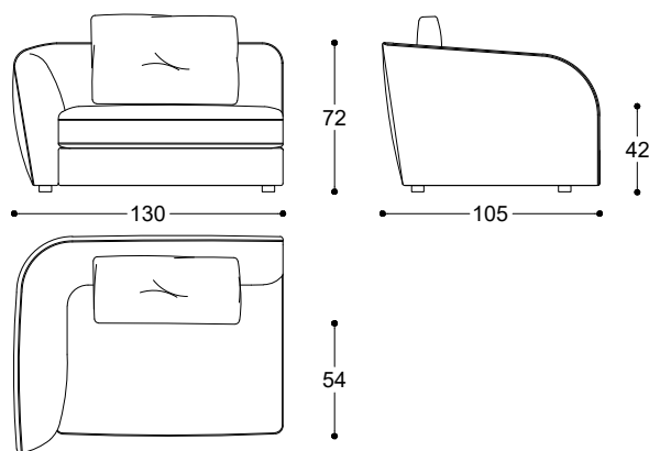
Article: Terminal element 130 Left Code: SX-LEV5H Article: Terminal element 130 Right Code: DX-LEV5G
