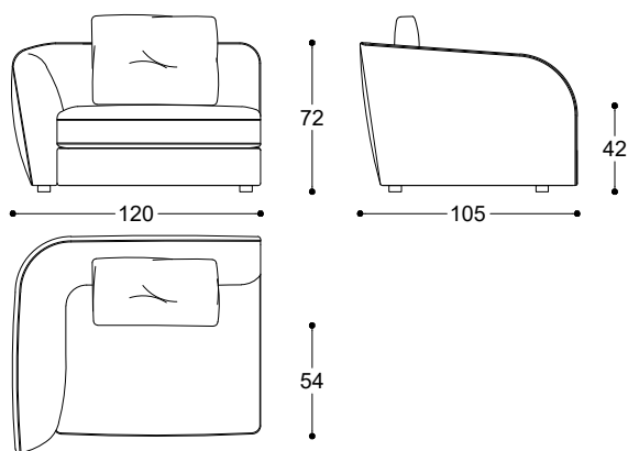
Article: Terminal element 120 Left Code: SX-LEV3F Article: Terminal element 120 Right Code: DX-LEV3E
