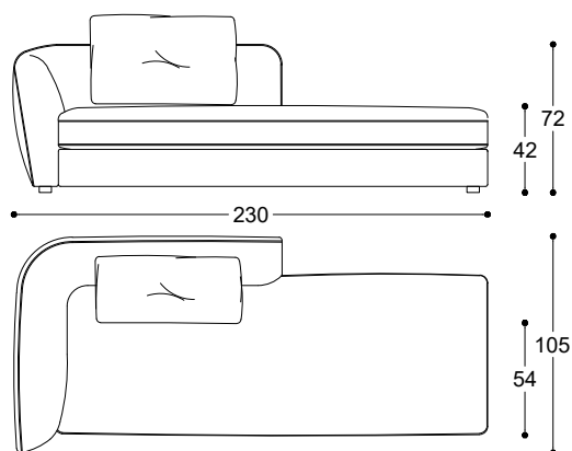
Article: Open terminal 230 Left Code: SX-LEV7P Article: Open terminal 230 Right Code: DX-LEV7N
