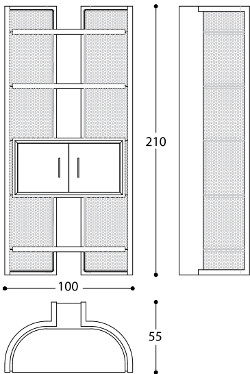
Article: Bookcase whit 3 shelves Code: BITO2 OPTIONS A B C D BITO2A BITO2B BITO2C BITO2D
